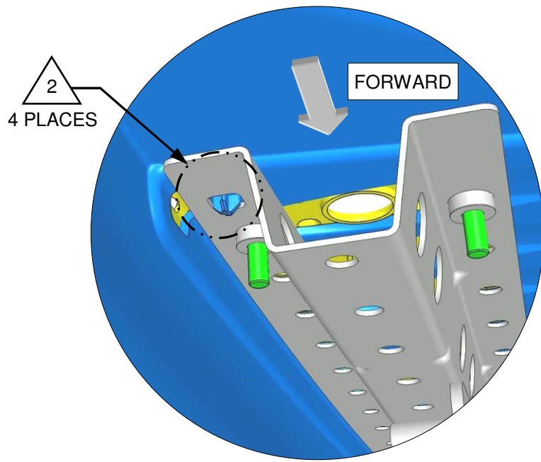
VIEW B
