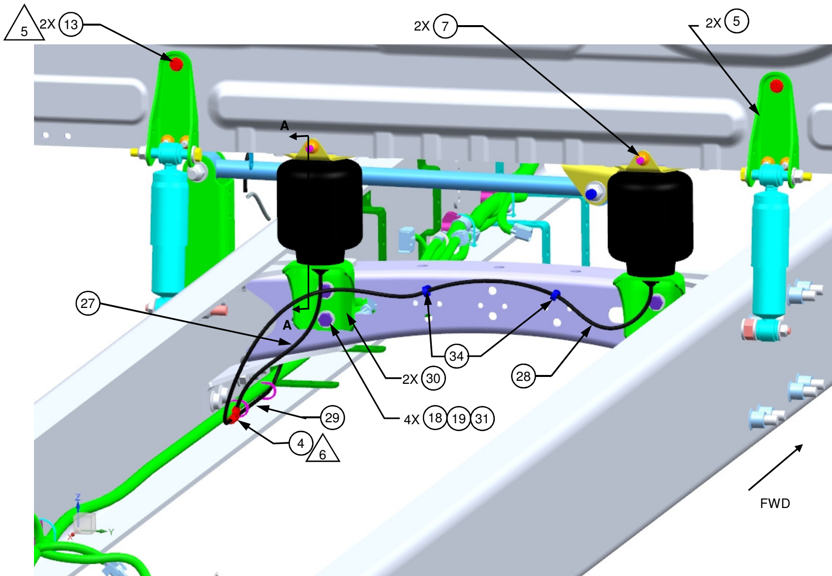
VIEW B
