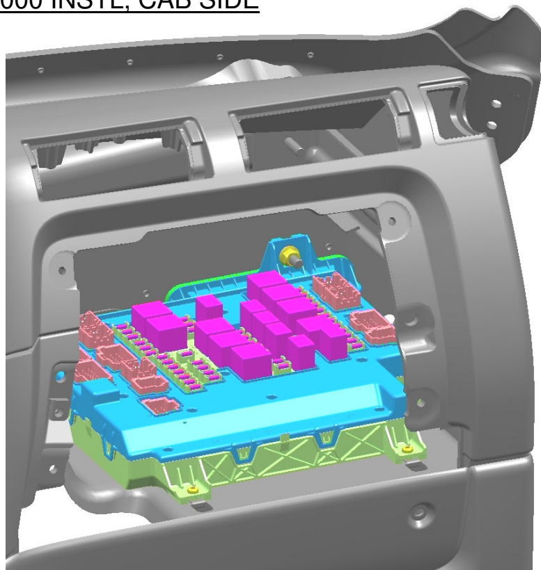
VIEW A HARDWARE IN PLACE
