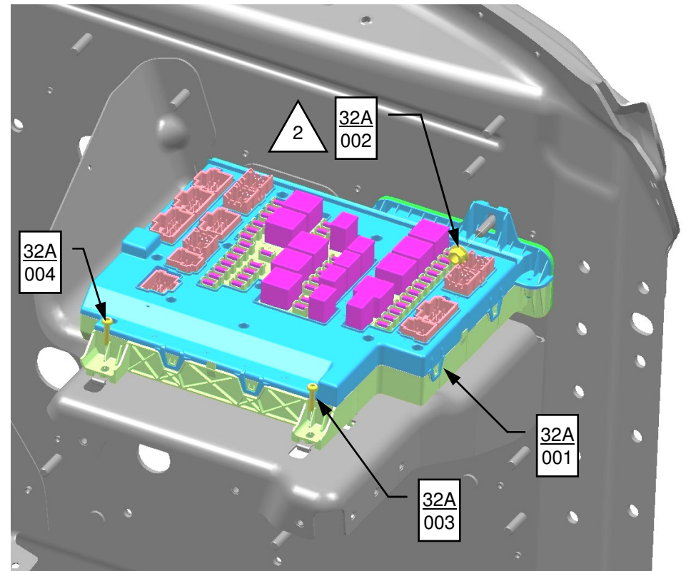
VIEW B HARDWARE EXPLODED SOME PARTS NOT SHOWN FOR CLARITY
